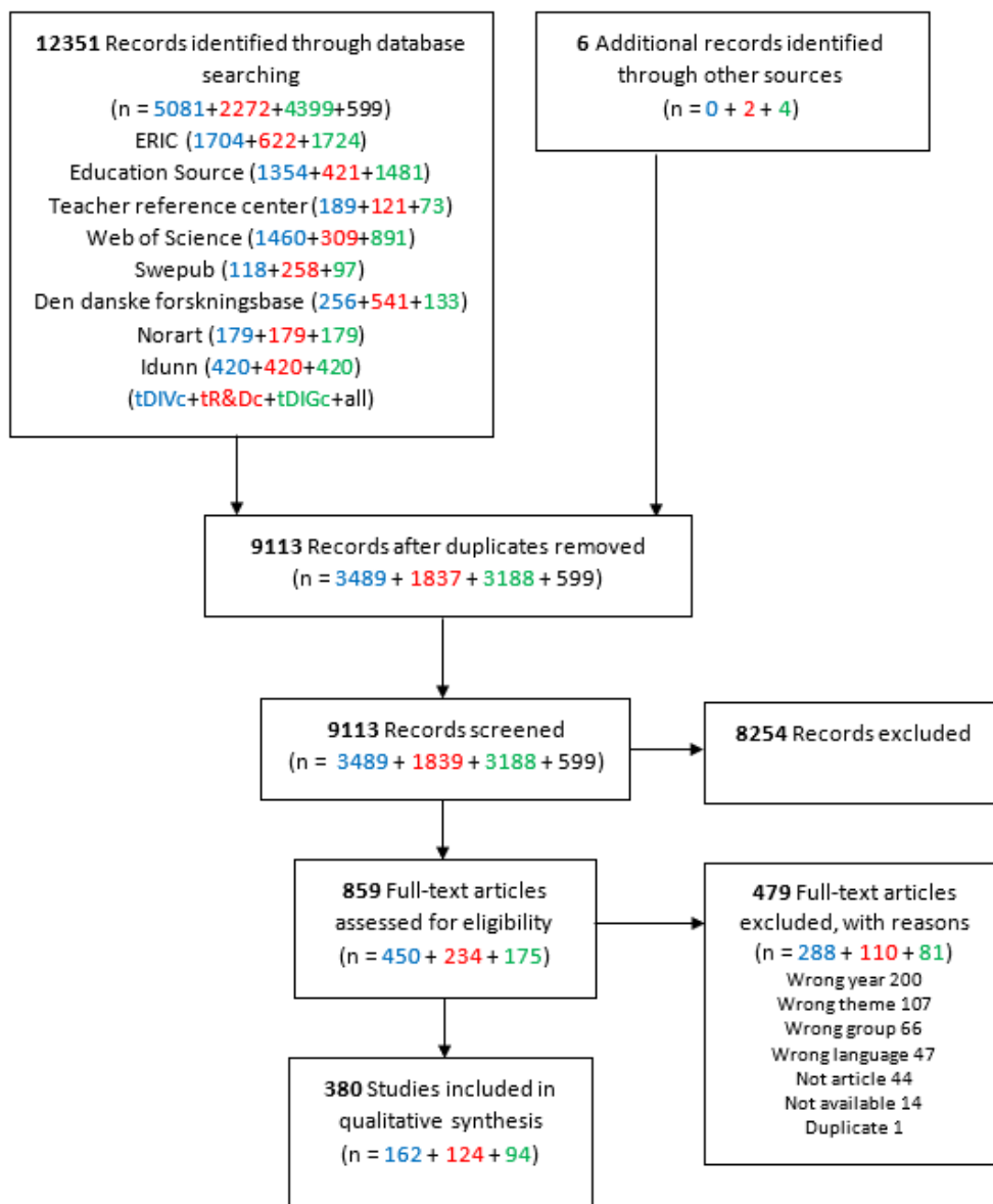
Figure 1. PRISMA diagram
